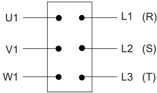
Panel connection
