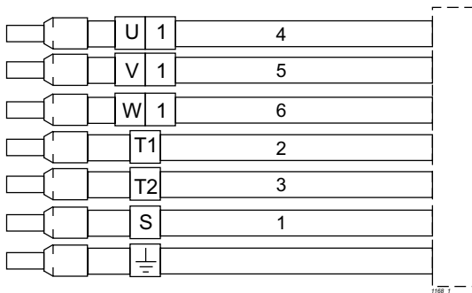
Electric pump cable conductor identification
